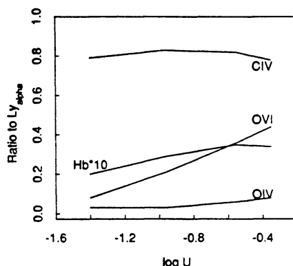
Figure 2: Line ratios vs. \log U .
