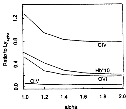
Figure 1: Line ratios vs. \alpha_{ox} .
