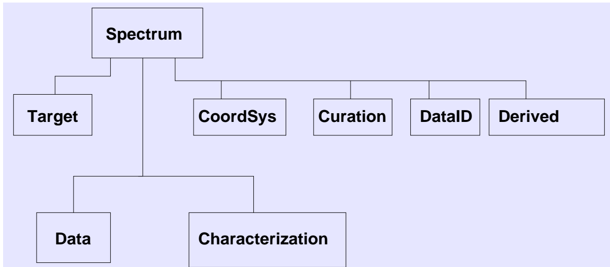
Figure 1: UML class diagram for the spectral data model. The Characterization, Curation, DataID and Derived classes are shown in detail below in diagram form and with further text description in Section 5.
